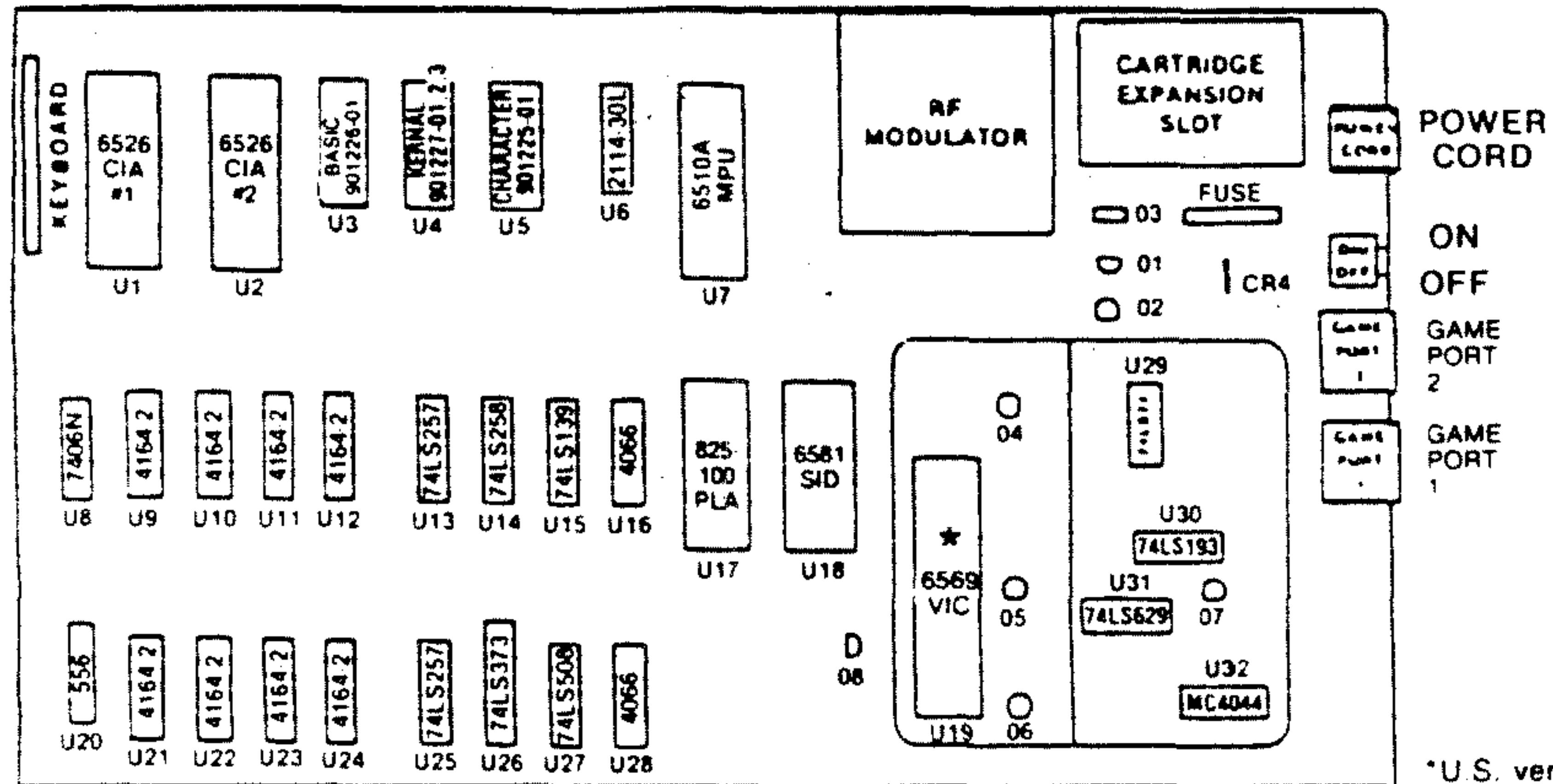
C-64 CHIP LAYOUT
