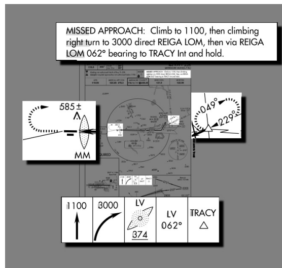
Abbildung 10.17: Missed approach procedure
