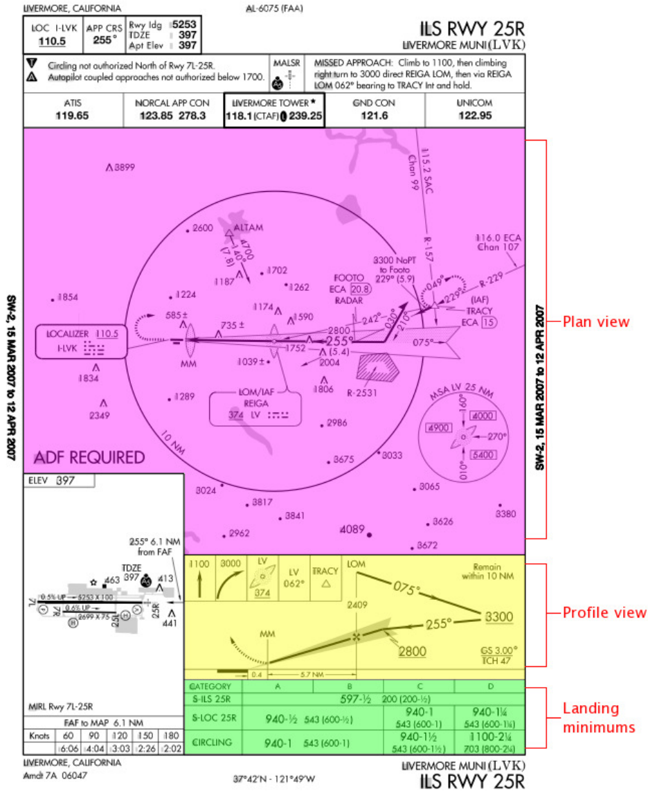
Abbildung 10.10: ILS approach plate for Livermore runway 25R
